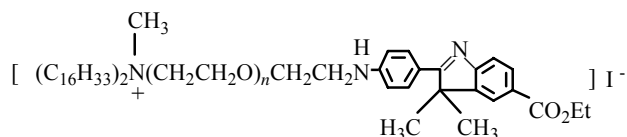
compound 1 , n=1 ; compound 2 , n=2 ; compound 3 , n=3
